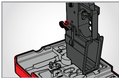
Holds lower in vertical position to remove 3/32" bolt catch roll pin.
