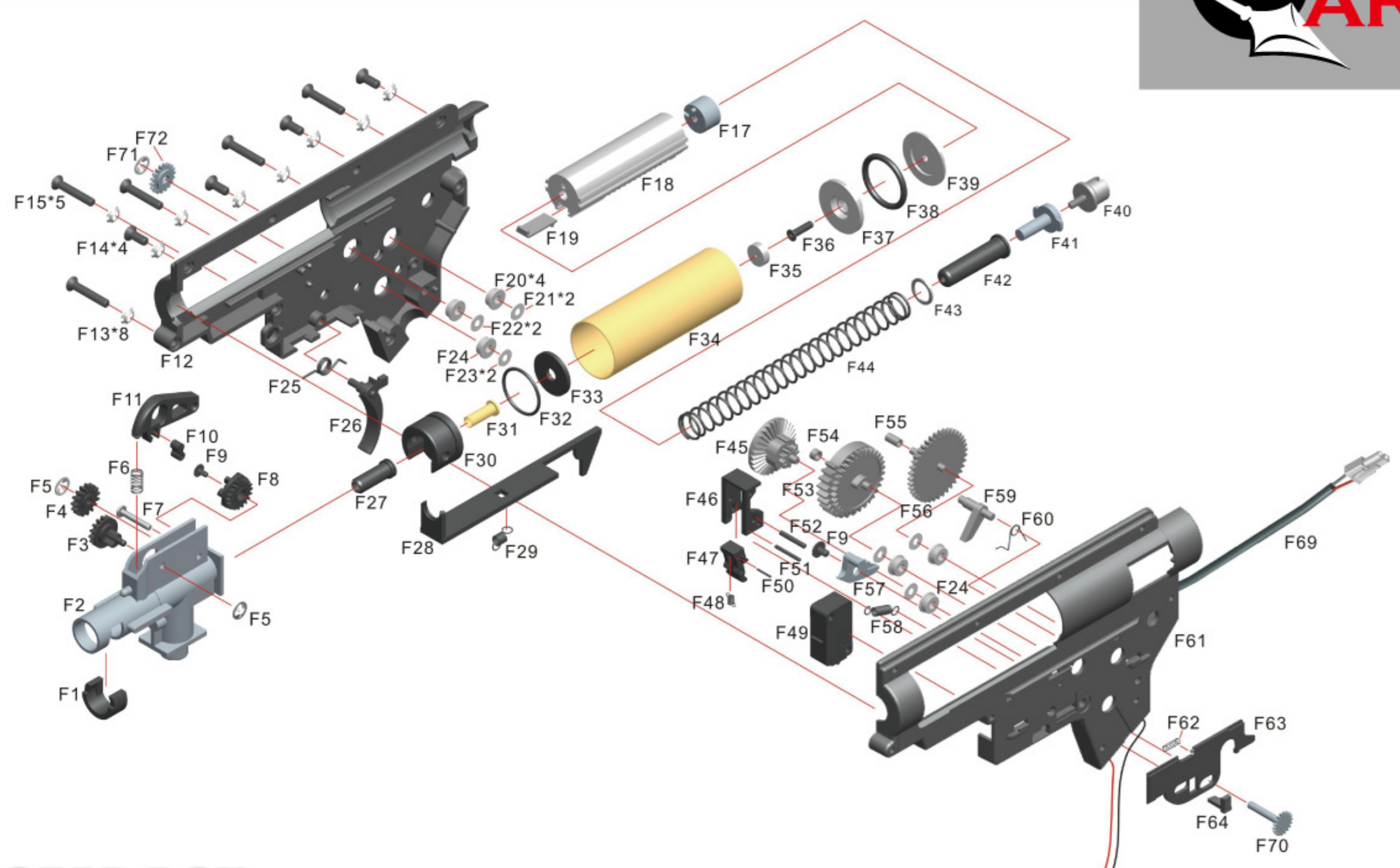
GEAR BOX
